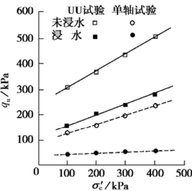
图 4 抗剪强度与围压关系 Fig. 4 Relationship between shear strength and consolidation pressure
