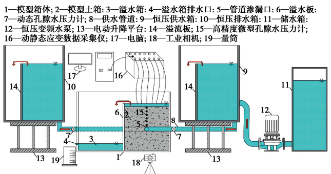
图 2 供水管道渗漏砂土诱发流化试验装置示意图 Fig. 2 Schematic diagram of sand induced fluidization test device for water supply pipeline leakage
