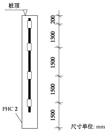
(c) PHC桩芯混凝土应力计布置
